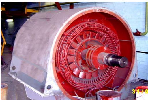
Motor: Synchronous, 1000 RPM, 10KV, 167A, 2.5MW.
